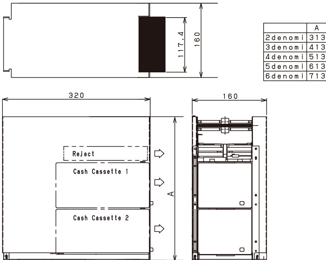
The Model F53 Specifications (2-Denominations)
